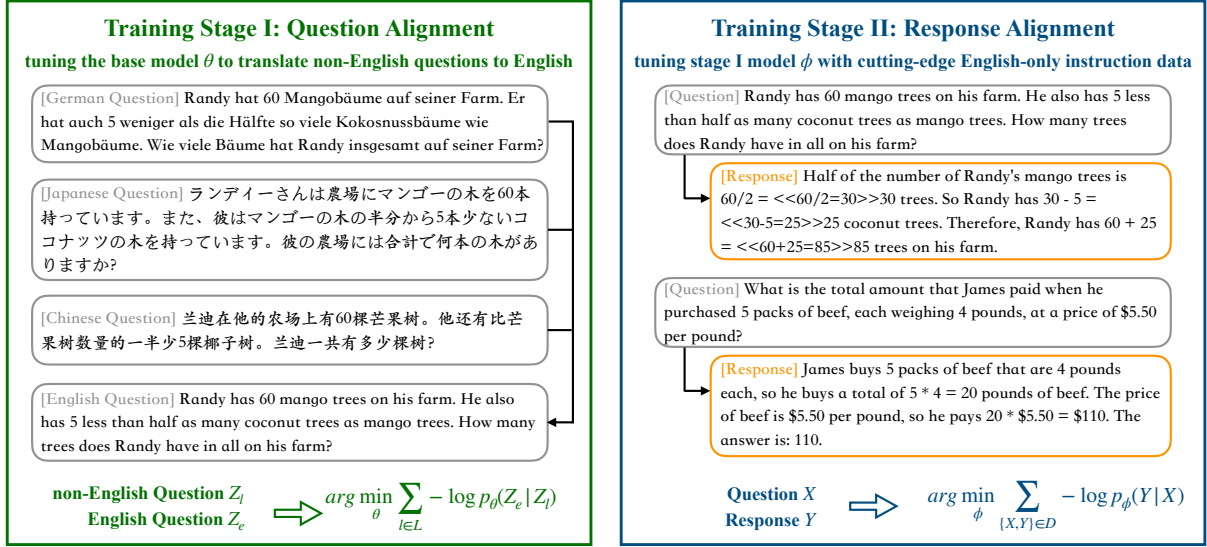
Figure 1: Illustration of our devised two-step training framework. At training stage I, we use a set of multilingual questions for translation training. At training stage II, we use cutting-edge English-only supervised data for fine-tuning. Due to the established language alignment in stage I, the LLM’s proficiency in English can be transferred to non-English tasks.
