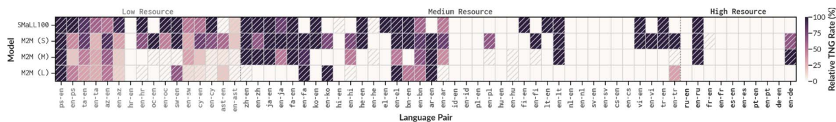
Figure 2: Heatmap of the rate of hallucinations detected with TNG (oscillatory hallucinations) among all hallucinations. Patterned cells indicate at least one natural hallucination for a given model-LP pair.
