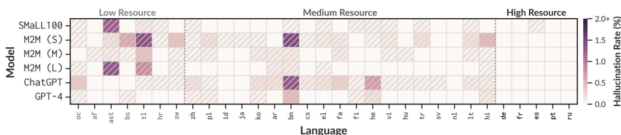
Figure 1: Hallucination rates among candidate translations for each model in the languages considered. Pattern-filled cells indicate at least one hallucination for a given model-language pair.
